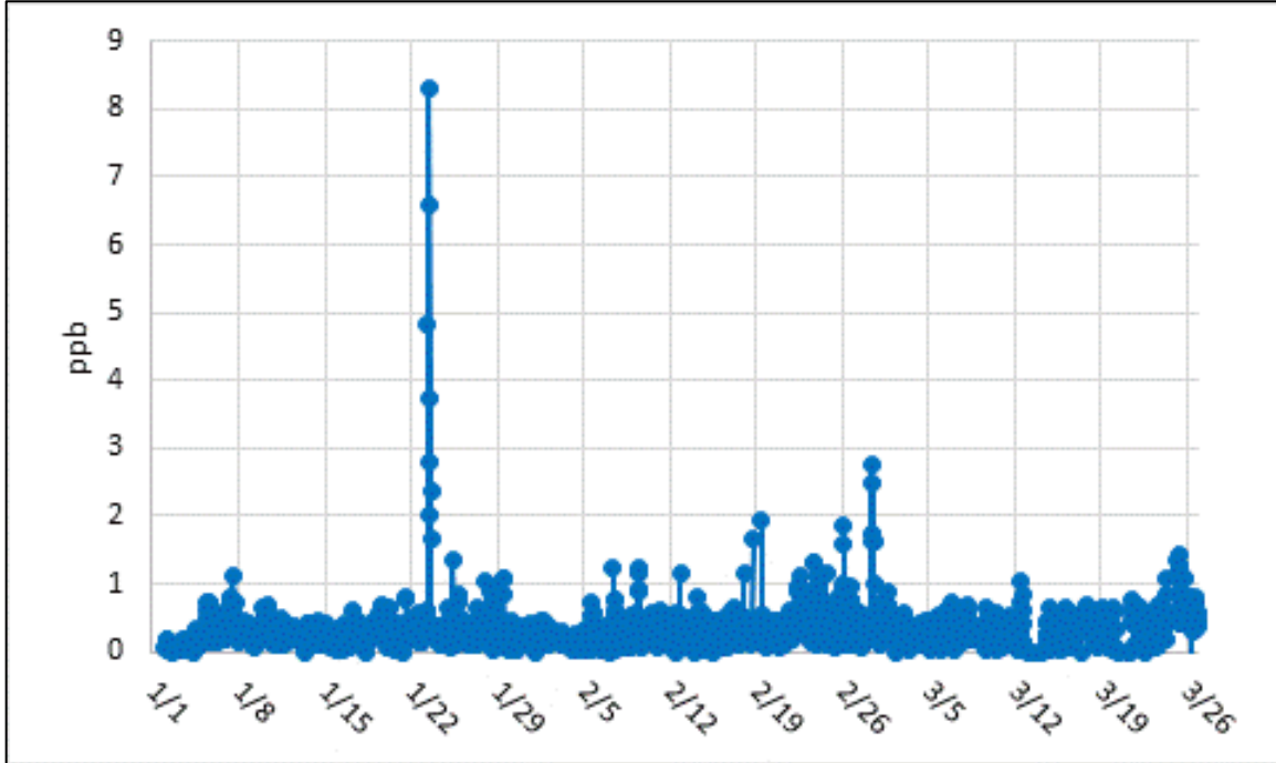
Figure 11. Hourly average SO 2 at GF, ppb units, Jan. 1 – Mar. 27, 2022
