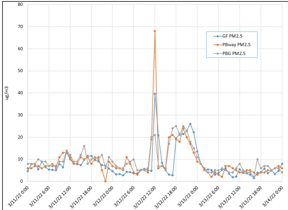
Figure 19. Nearly coincident elevated PM2.5 on Mar. 12, 2022, northerly winds
