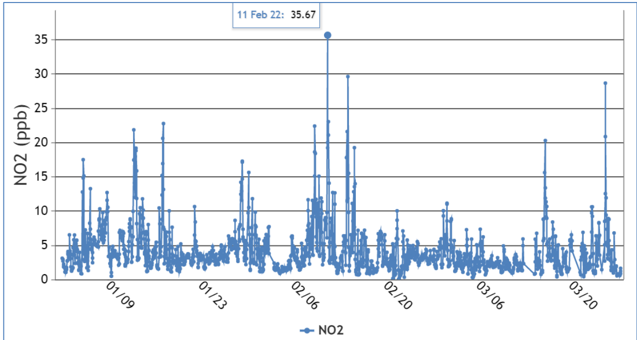
Figure 9. Hourly NO 2 at GF, ppb units, Jan. 1 – Mar. 27, 2022
