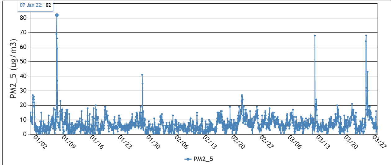
Figure 14. Hourly average PM2.5 at PBway, \mu\text{g}/\text{m}^3 , Jan. 1 – Mar. 27, 2022
