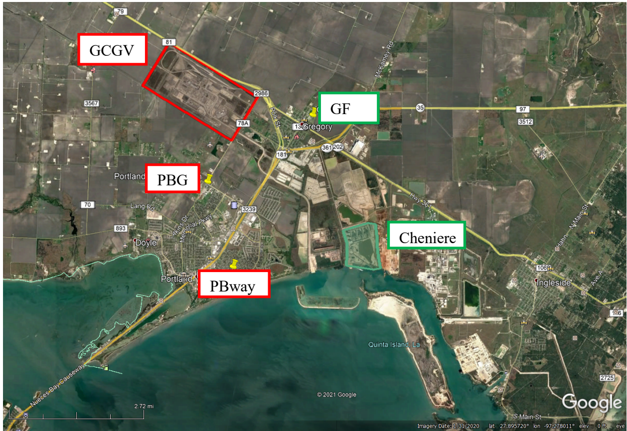
Figure 22. Location of Gregory-Fresno Community Air Monitoring Station (GF), and two Portland community stations on GPISD campuses on Buddy Ganem (PBG) and on Broadway (PBway) and the Cheniere Energy and GCGV industrial facilities
