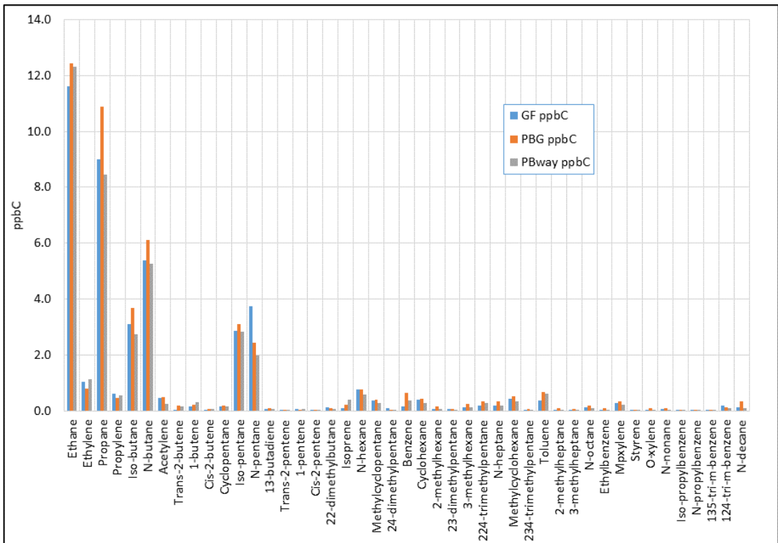
Figure 6. Calendar year 2021 mean concentrations of hydrocarbon species at the three air monitoring stations
