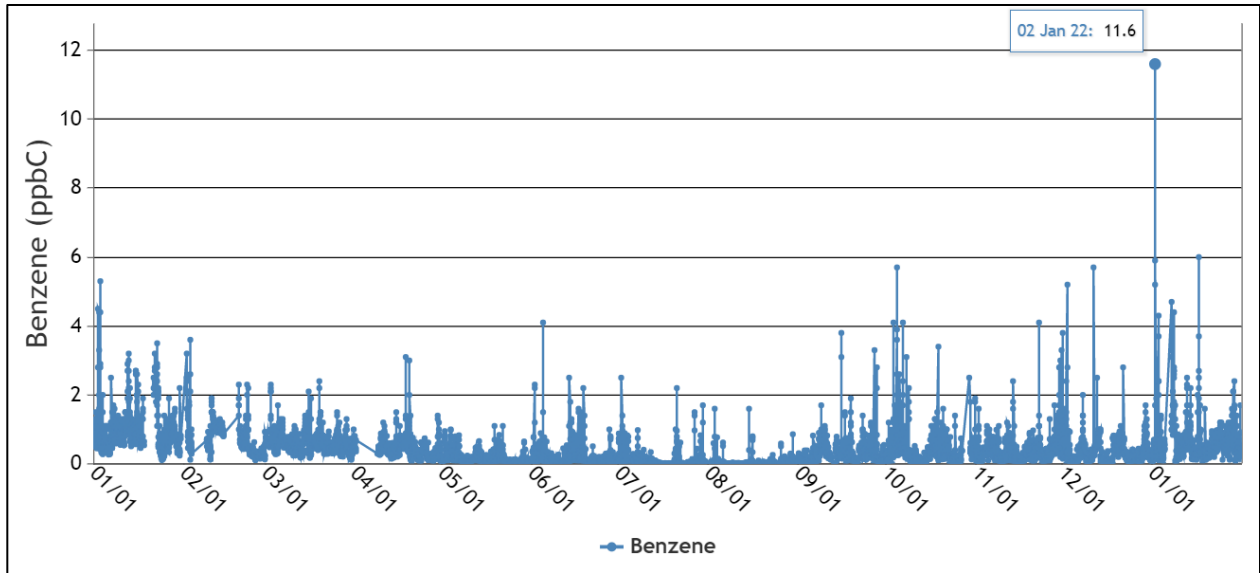
Figure 4. Hourly benzene concentrations at PBway station, Jan. 1, 2021 – Jan. 31, 2022, ppbC units
