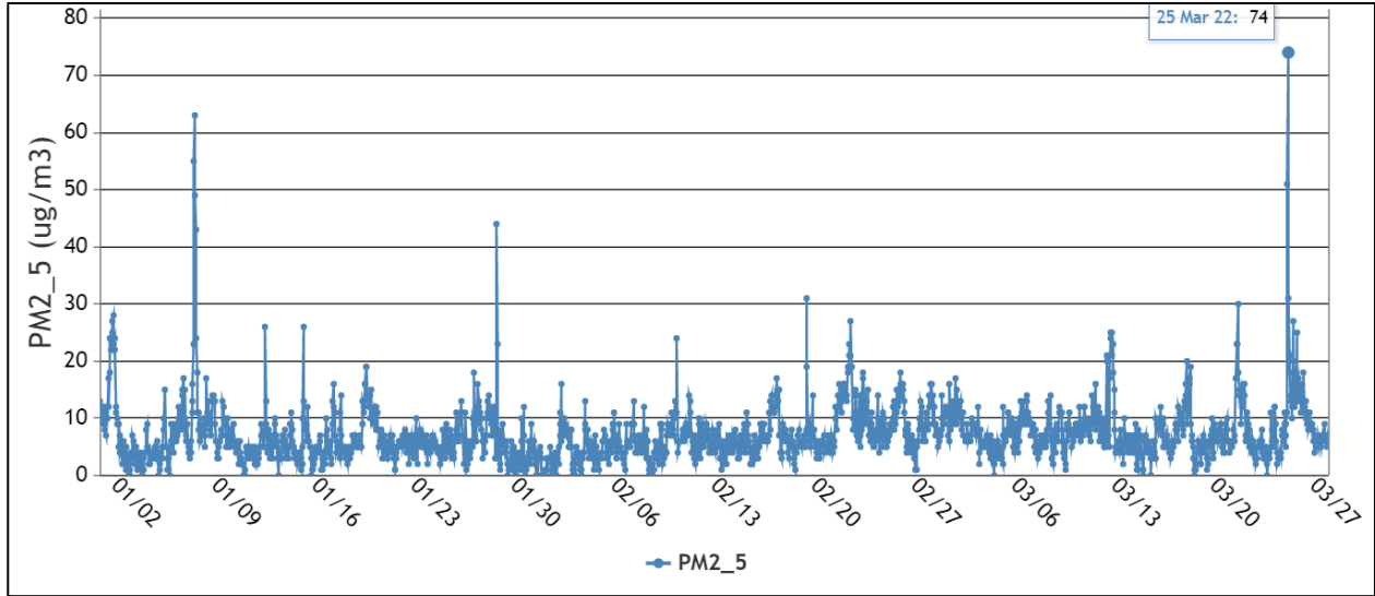
Figure 12. Hourly average PM2.5 at PBG, µg/m 3 , Jan. 1 – Mar. 27, 2022
