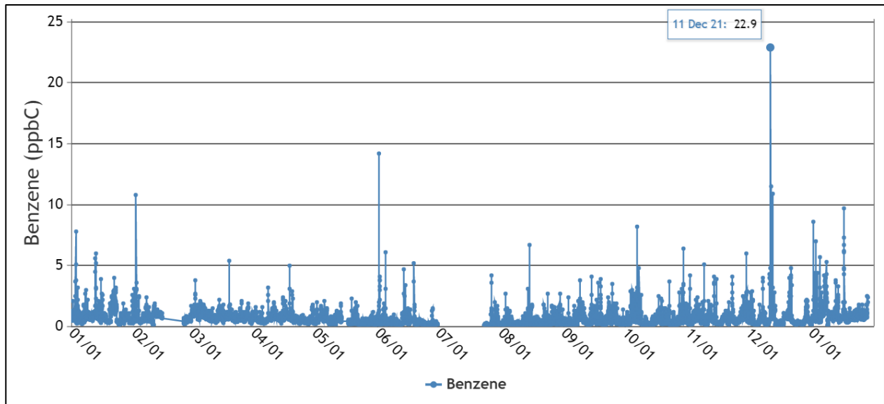
Figure 3. Hourly benzene concentrations at PBG station, Jan. 1, 2021 – Jan. 31, 2022, ppbC units
