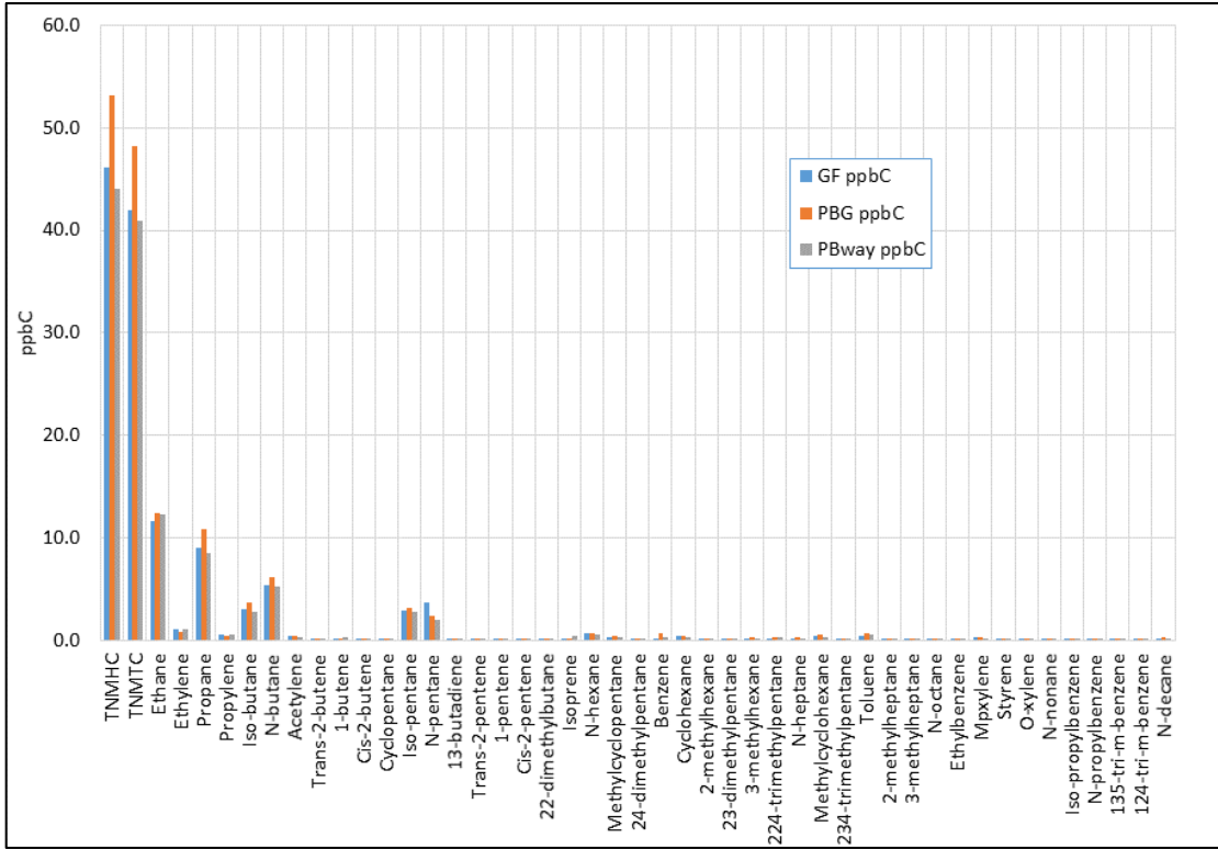
Figure 5. Calendar year 2021 mean concentrations of TNMHC, TNMTC, and hydrocarbon species at three stations
