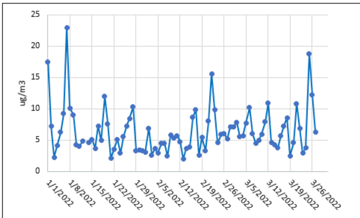
Figure 8. Averaged 24-Hour PM2.5 at GF, \mu\text{g}/\text{m}^3 , Jan. 1 – Mar. 26, 2022
