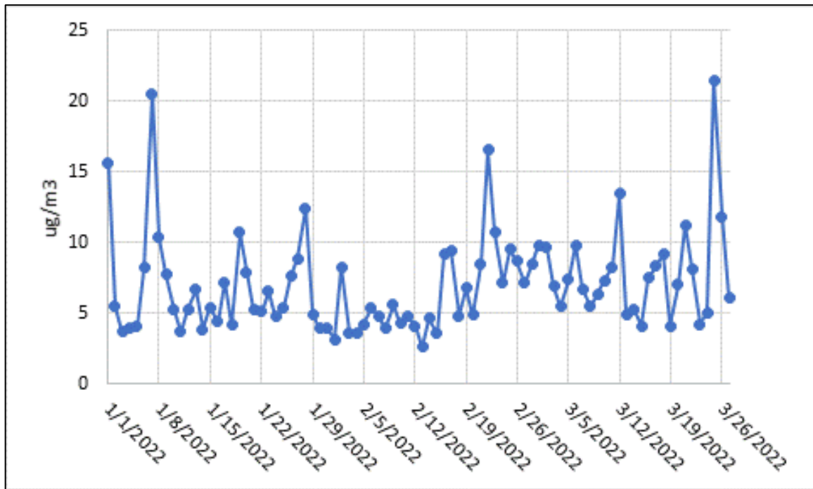
Figure 15. Averaged 24-Hour PM2.5 at PBway, \mu\text{g}/\text{m}^3 , Jan. 1 – Mar. 27, 2022
