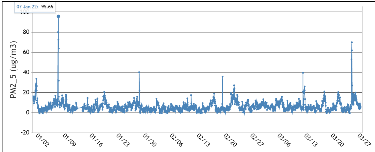
Figure 7. Hourly average PM2.5 at GF, \mu\text{g}/\text{m}^3 , Jan. 1 – Mar. 27, 2022
