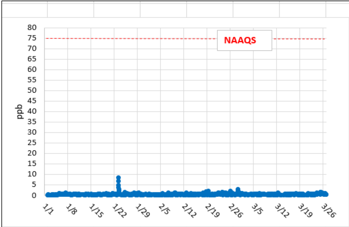
Figure 10. Hourly average SO 2 at GF, ppb units, Jan. 1 – Mar. 27, 2022, NAAQS scale
