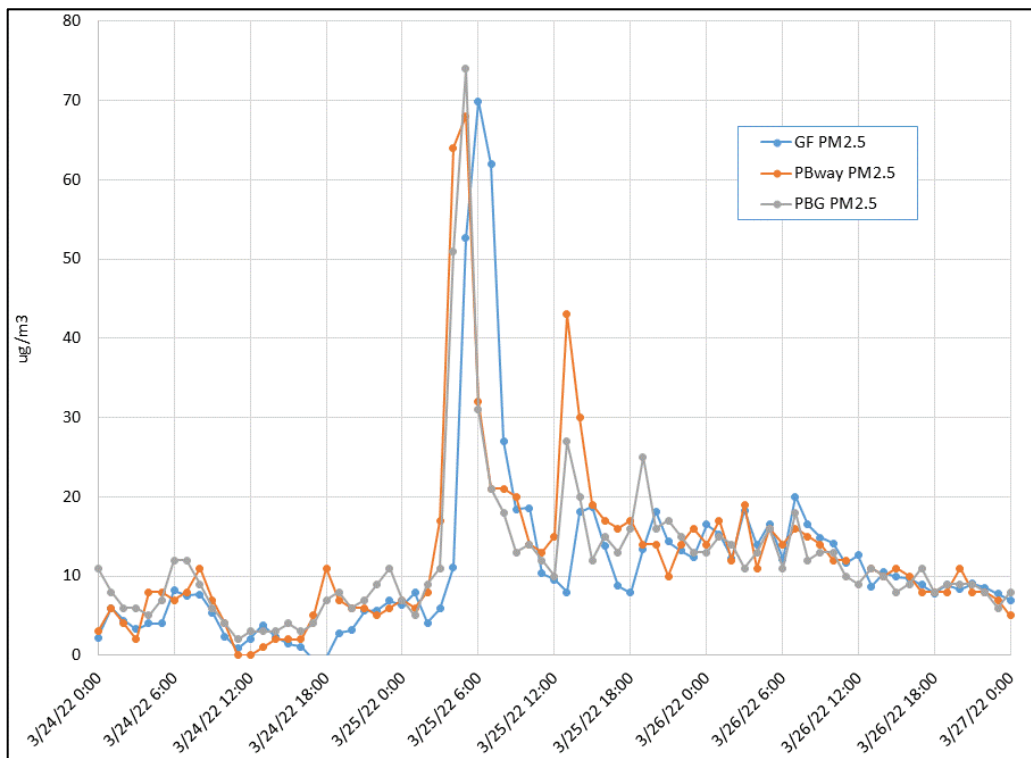
Figure 20. Nearly coincident elevated PM2.5 on Mar. 25, 2022, southerly winds
