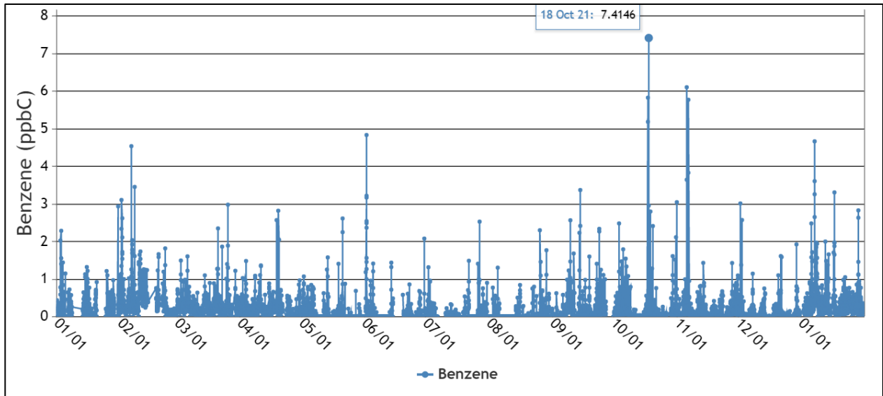
Figure 2. Hourly benzene concentrations at GF station, Jan. 1, 2021 – Jan. 31, 2022, ppbC units
